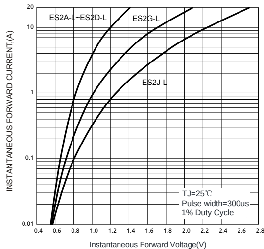
FIG.3-TYPICAL FORWARD CHARACTERISTICS
